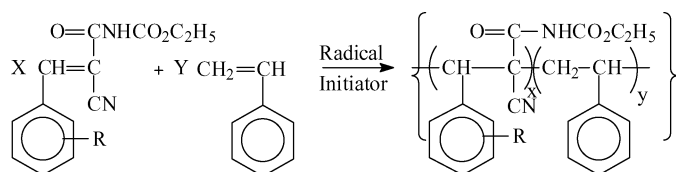
Sch. 1. Copolymer synthesis (where R is 2,3,4-(CH 3 O) 3 , 2,4,5-(CH 3 O) 3 , 2,4,6-(CH 3 O) 3 , 3,4,5-(CH 3 O) 3 , 2,3-(CH 3 ) 2 and 4-CH 3 O).
